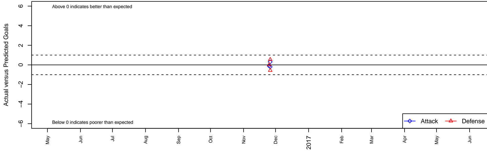
Granite Fall Hydro B98 Dots are actual minus expected GF (blue circles) and GA (red triangles). Blue line is smoothed change in attack strength. Red is smoothed change in defense strength.
